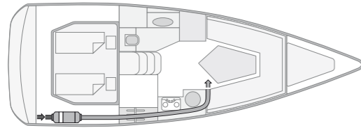
For small boats with only one main cabin, one non-closable outlet is fully sufficient.
